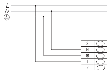
DALI-CASAMBI (3 core cable) 5P 230 V
