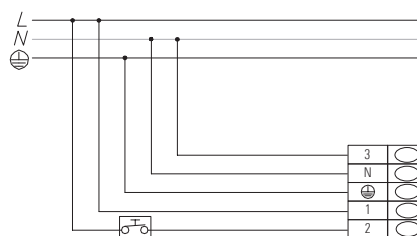
DALI - touch dim (5 core cable) 5P 230 V Single push for direct and indirect illumination
