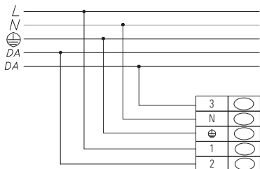
DALI (5 core cable) 5P 230 V
