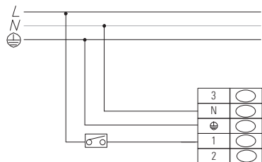
FO (3 core cable) 5P 230 V
