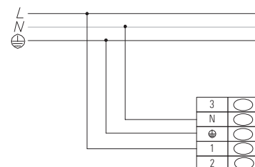
DALI-CASAMBI (3 core cable) 5P
