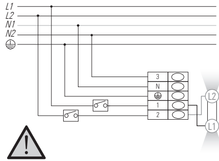
FO - double switch (5 core cable) 5P 230 V
