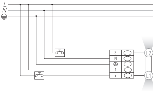
TD - touch dim double switch (5 core cable) 5P 230 V
