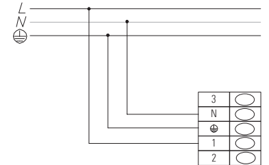
DALI-CASAMBI (3 core cable) 5P 230 V
